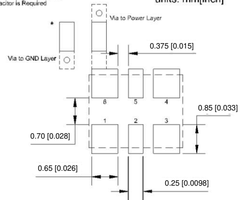
Recommended Solder Pad Layout units: mm[inch]
