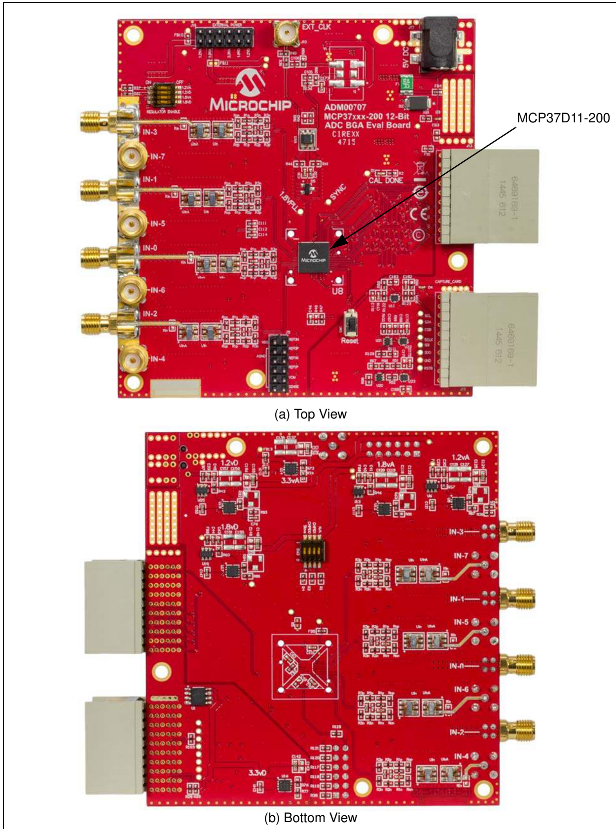
FIGURE 1-2: MCP37X1X-200 12-Bit 200 Mps ADC BGA Evaluation Board (ADM00707).
