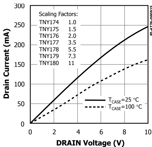
Figure 22. Output Characteristic.
