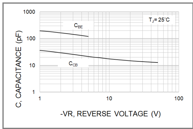
Fig.6 Typical Capacitance
