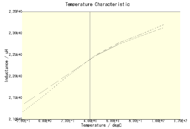
CLF7045T-2R2N-CA(DC = 0A)
