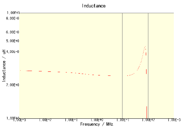
CLF7045T-2R2N-CA
