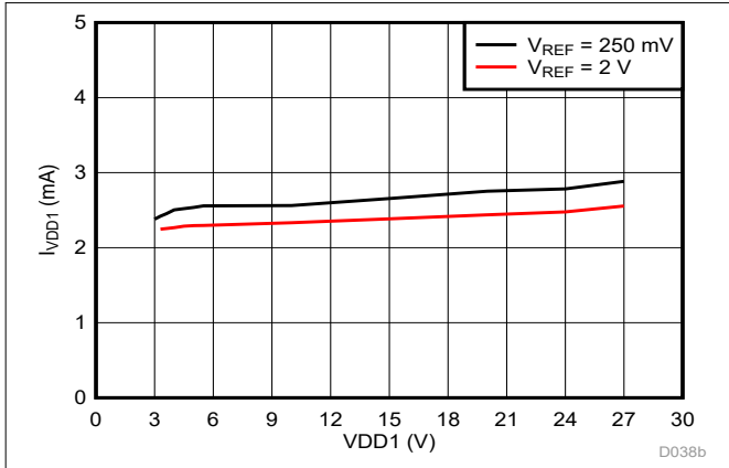
Figure 6-29. High-Side Supply Current vs Supply Voltage
