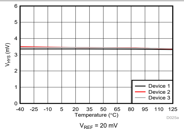
Figure 6-10. Trip Threshold Hysteresis vs Temperature
