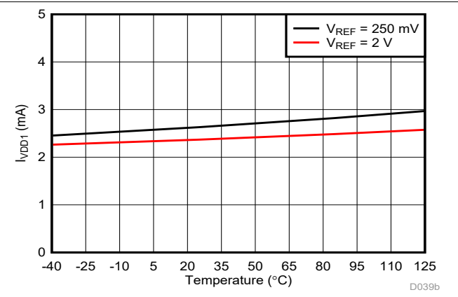
Figure 6-30. High-Side Supply Current vs Temperature
