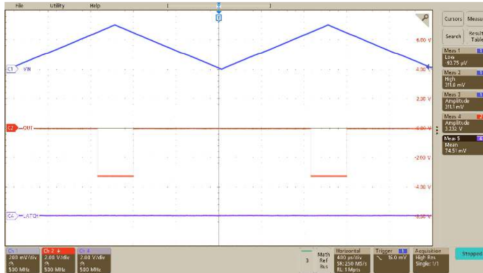
Figure 8-2. Output Response of the AMC23C11-Q1 to a Triangular Input Waveform
