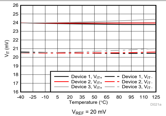
Figure 6-6. Trip Threshold vs Temperature
