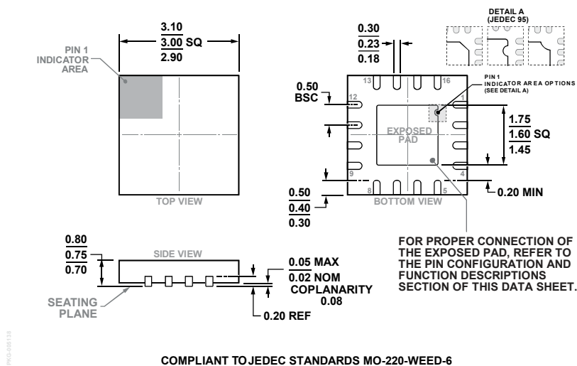
Figure 47. 16-Lead Lead Frame Chip Scale Package [LFCSP] 3 mm × 3 mm Body and 0.75 mm Package Height (CP-16-22)
