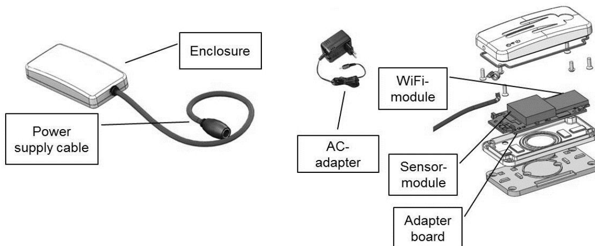
Figure 1 SCA11H assembly
