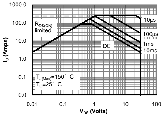
VGS > or equal 4.5V Figure 9: Maximum Forward Biased Safe Operating Area (Note F)
