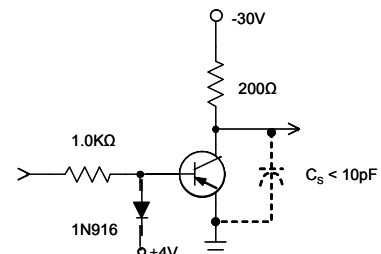
Fig. 2. Turn-Off Time
