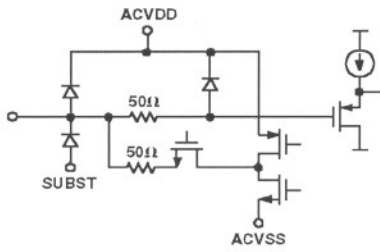
Figure 11. Pin 34 (AUXIN) and Pin 36 (ADCIN)
