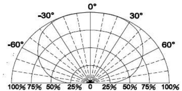
Fig.6 Directive Radiation
