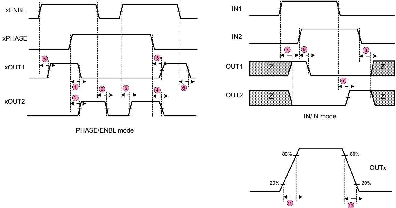
Figure 1. Timing Requirements
