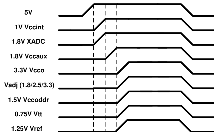
Figure 18 - Power Sequencing
