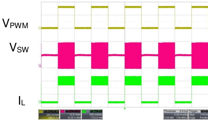
R_S Short ( V_{LED}=9\text{V} , R_S=0.3\Omega , L=47\mu\text{H} )
