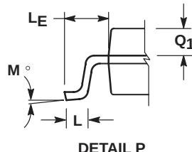
DETAIL P
