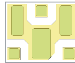
Figure 25. Solder stencil overlaid on AMCD-7602 bottom metal pattern
