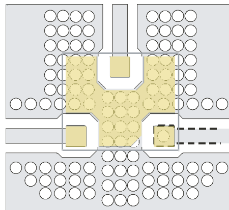
Figure 21. ACMD-7602 superposed on PCB layout
