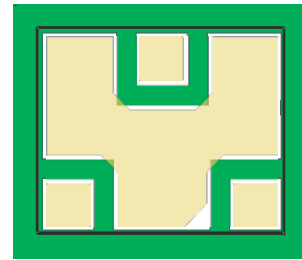
Figure 23. AMCD-7602 superposed on solder mask
