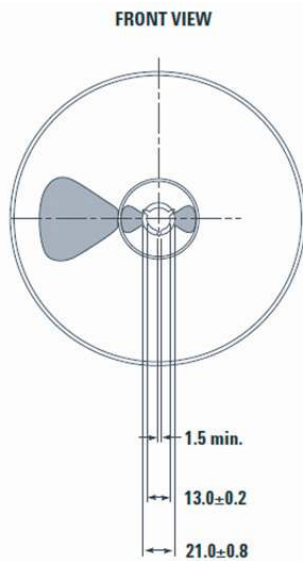
Figure 29. Reel drawing, front view
