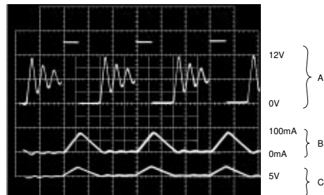
MAX758A SWITCHING WAVEFORMS DISCONTINUOUS CONDUCTION
