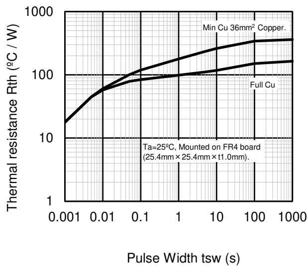
Rth - tsw
