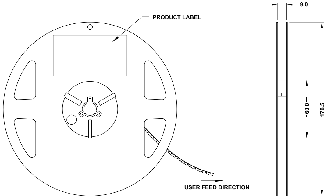
Figure 21: Reel Dimensions
