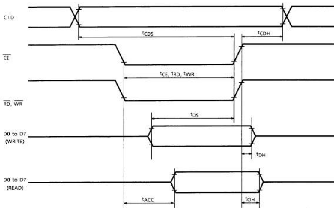
Figure 4: Timing Waveform
