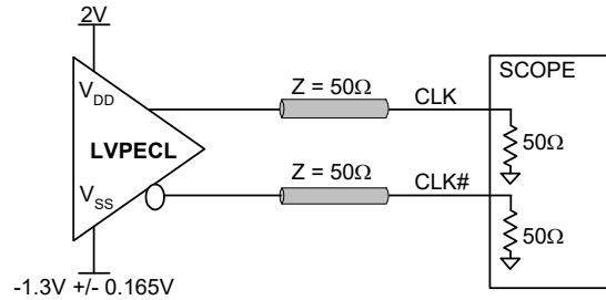
Figure 6. 2.5 V Output Load AC Test Circuit
