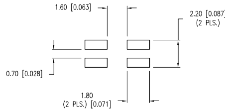
D C RECOMMENDED SOLDER PAD LAYOUT
