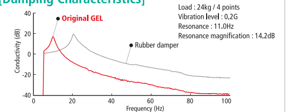
[Damping Characteristics]
