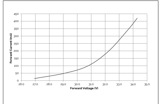
Figure 2: 12W Forward Voltage vs. Forward Current, T_c=25^\circ\text{C}
