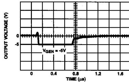
FIGURE 9F. V_{OUT} vs TIME
