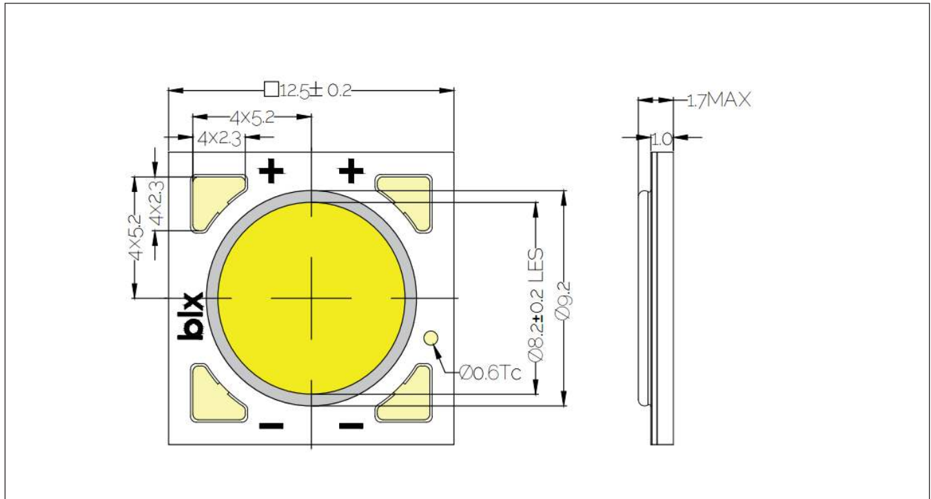
Figure 20: V8 LED Array
