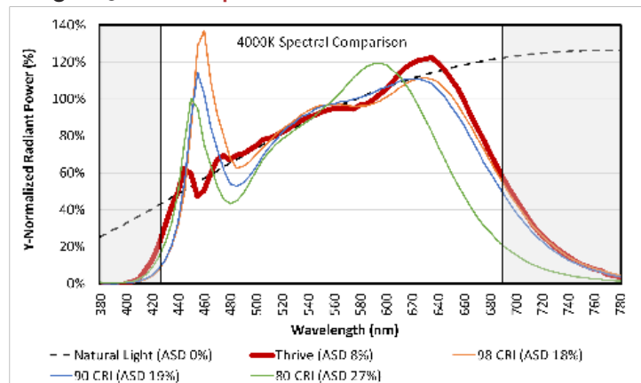
Figure 9: SPD Comparison
