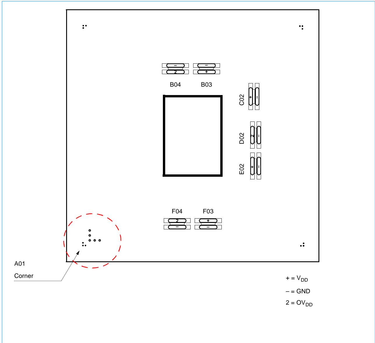
Figure 4-3. Module Substrate Decoupling Voltage Assignments
