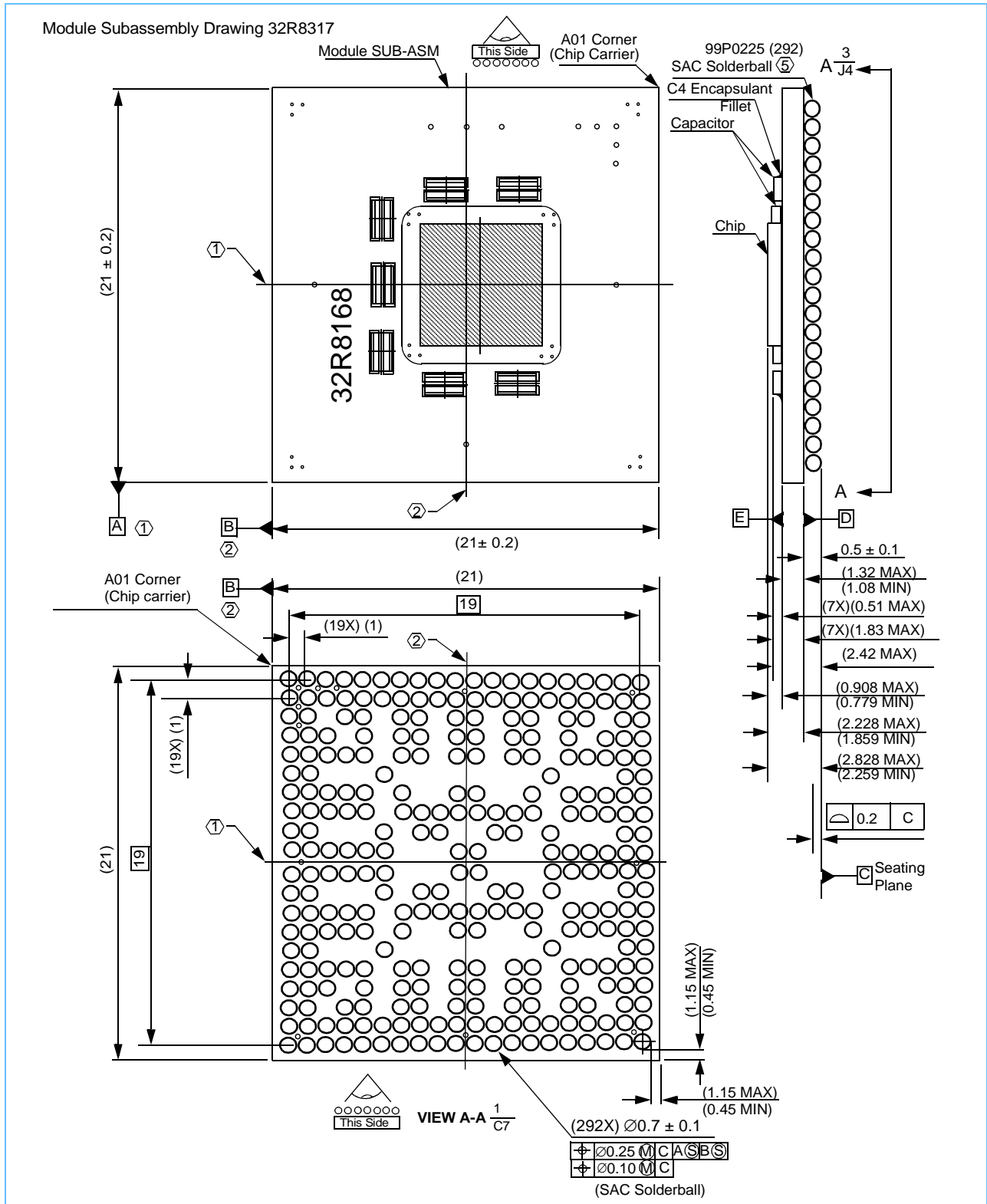
Figure 4-2. Mechanical Dimensions, ROHS-Compatible Package
