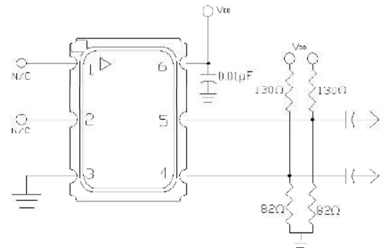
Figure 7. Pull-Up Pull Down Termination Resistor values shown are typical for 3.3 V operation. For 2.5V operation, the resistor to ground is 62 ohms and the resistor to supply is 250 ohms
