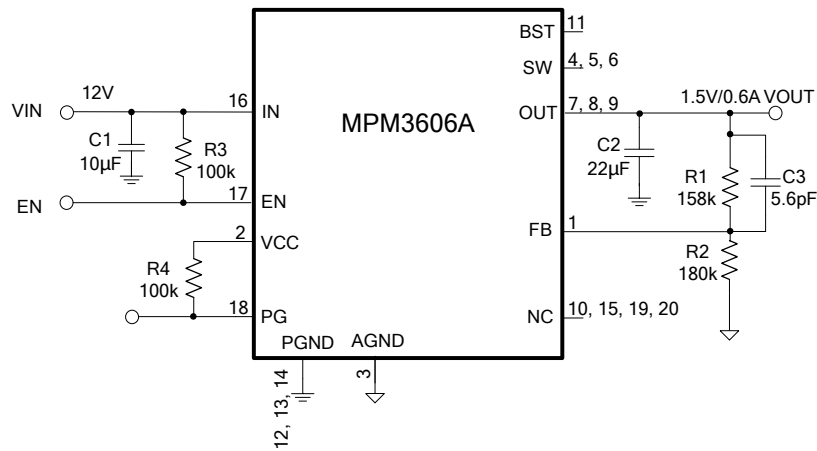
Figure 13. V_o=1.5V , I_o=0.6A
