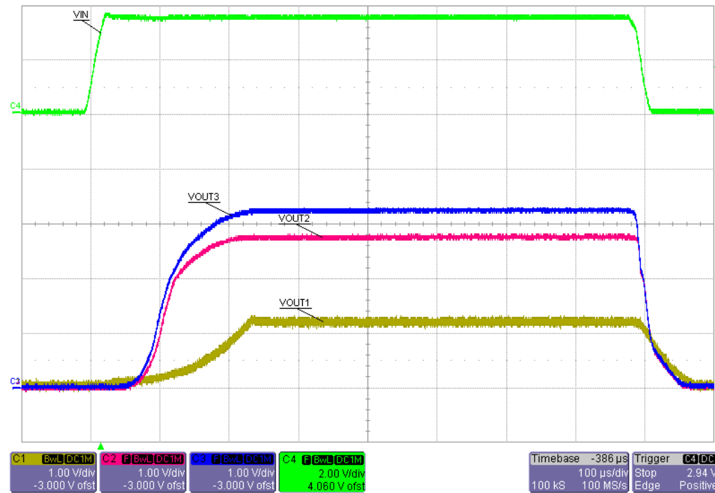
Figure 5. Startup and Shutdown with VIN Applied and Removed (ILOAD = 0.5*I max for all outputs, ENx = VIN).
