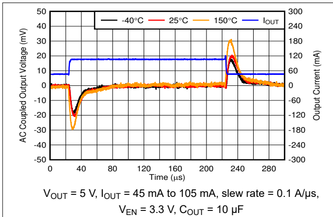
Figure 6-19. Load Transient, 45 mA to 105 mA
