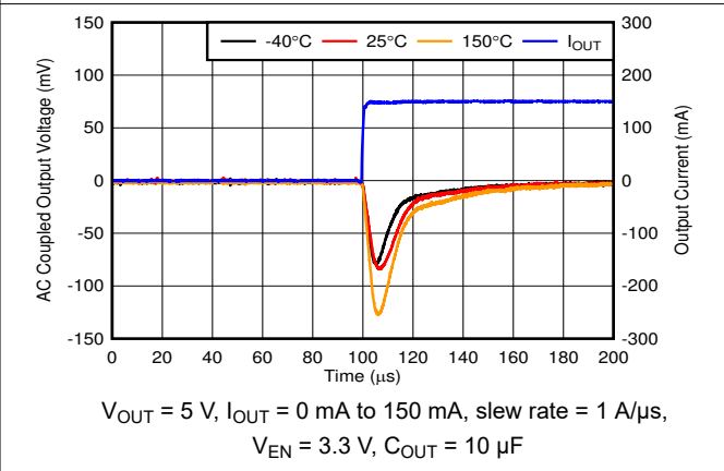
Figure 6-22. Load Transient, No Load to 150-mA Rising Edge
