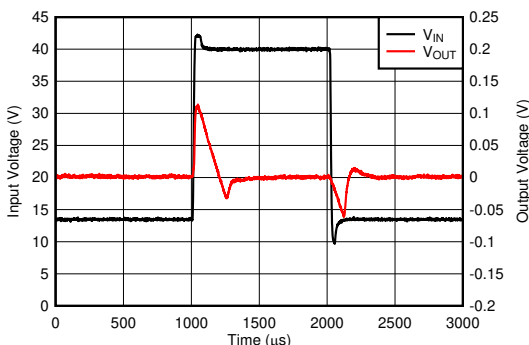
Line Transient Response ( 3\text{-V}/\mu\text{s} V_{IN} Slew Rate)
