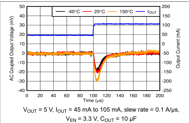
Figure 6-20. Load Transient, 45-mA to 105-mA Rising Edge
