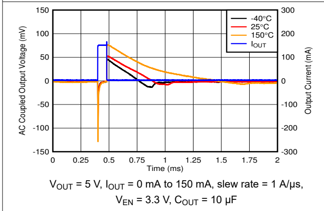
Figure 6-21. Load Transient, No Load to 150-mA
