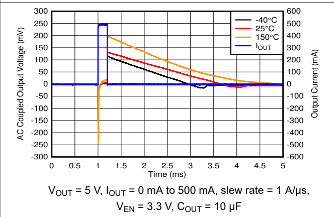
Figure 6-24. Load Transient, No Load to 500 mA
