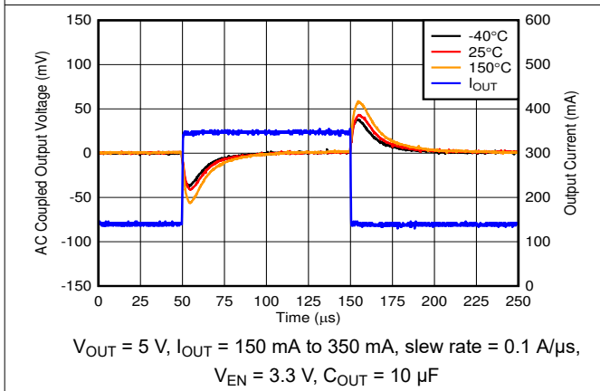
Figure 6-23. Load Transient, 150-mA to 350-mA
