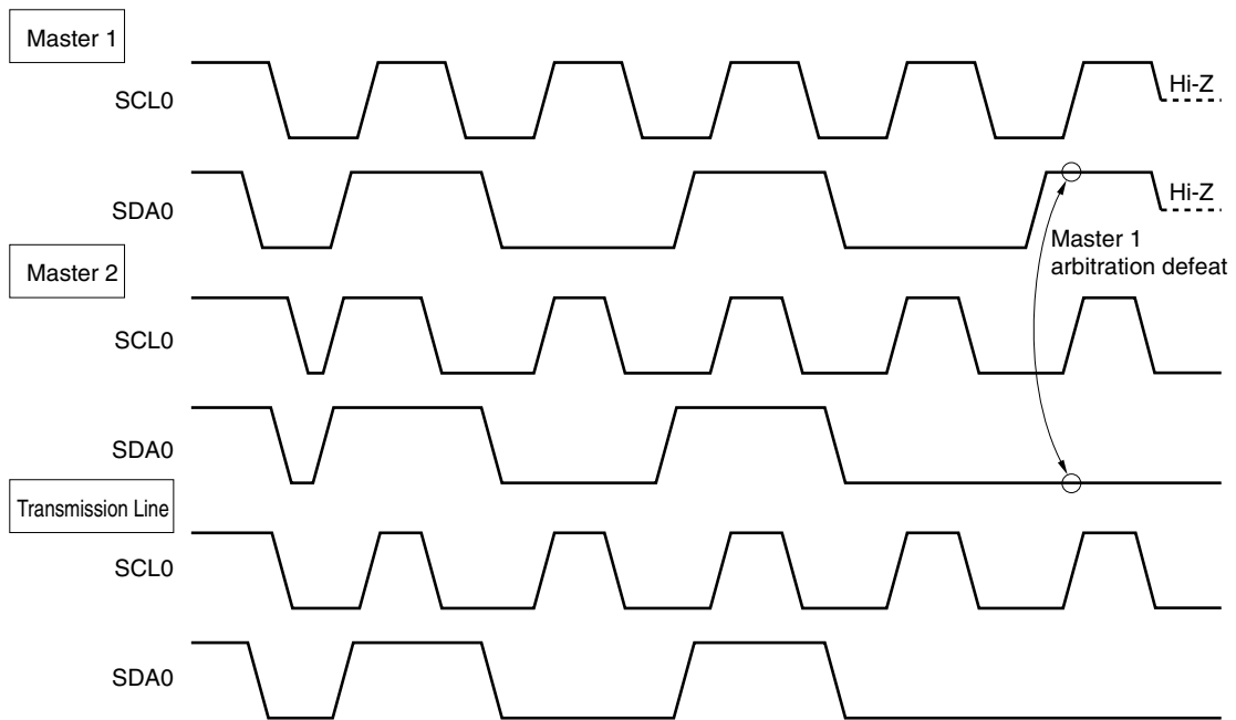
Figure 15-14. Arbitration Timing Examples
