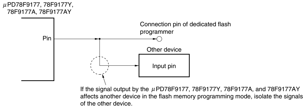
Figure 20-6. Abnormal Operation of Other Device
