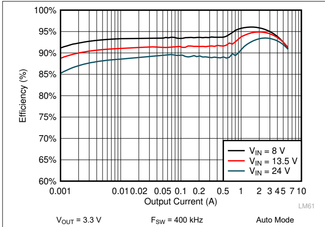
Figure 9-5. LM61460 Efficiency
