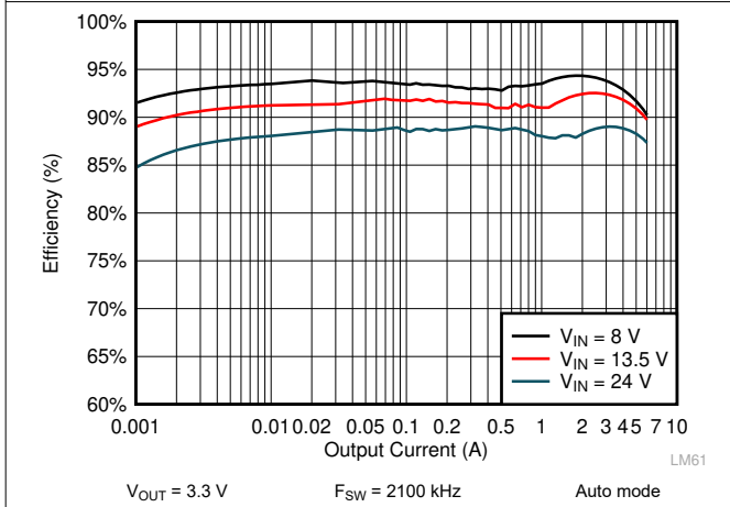
Figure 9-9. LM61460 Efficiency
