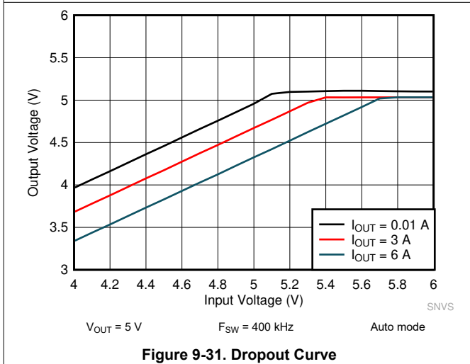
Figure 9-31. Dropout Curve
