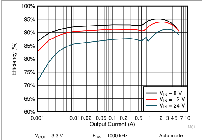
Figure 9-7. LM61460 Efficiency
