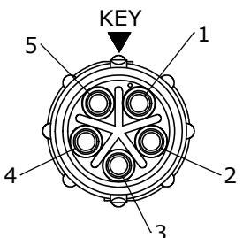
WIRE VIEW W8380-5PG-P-3XX
