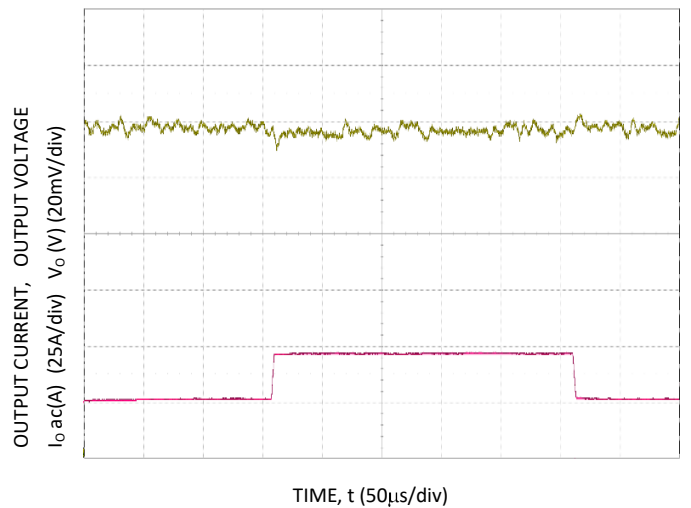
Figure 16. Trans. Resp. to 10A/μs Load Change from 25% to 75% at 12V IN , C o = 4x0.047μF + 4x0.1μF + 15x22μF + 73x47μF + 6x470μF polymer
