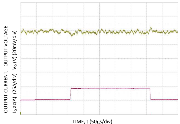
Figure 22. Trans. Res. to 10A/μs Load Change from 25% to 75% at 12V IN , C_o=4 \times 0.047\mu\text{F} + 4 \times 0.1\mu\text{F} + 15 \times 22\mu\text{F} + 73 \times 47\mu\text{F} + 6 \times 470\mu\text{F} polymer
