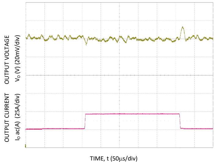
Figure 4. Trans. Resp. to 10A/ \mu\text{s} Load Change from 25% to 75% at 12VIN, C_o=4 \times 0.047 \mu\text{F} + 4 \times 0.1 \mu\text{F} + 15 \times 22 \mu\text{F} + 73 \times 47 \mu\text{F} + 6 \times 470 \mu\text{F} polymer
