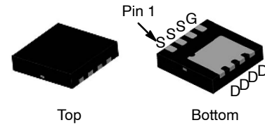
WDFN8 3.3 × 3.3, 0.65P CASE 511DH
