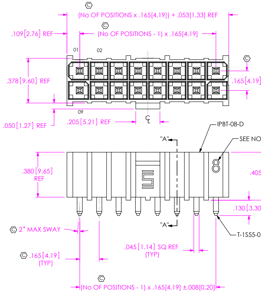
FIG. 1 (IPBT-108-H1-XX-D SHOWN)
