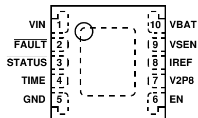
ISL9203 (3x3 DFN) TOP VIEW
