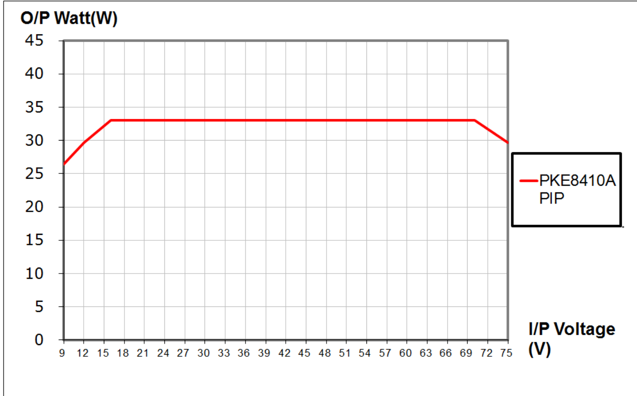
Note 2: PKE8410A PIP Power Derating Curve (Output Power VS Input Voltage)
