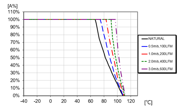
Available load current vs. ambient air temperature and airflow at V_1 = 48\text{ V} . See Thermal Consideration section.
