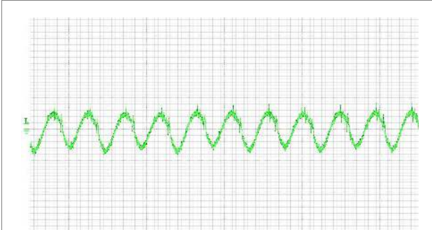
Output voltage ripple at: T_{P1} = +25^{\circ}\text{C} , V_i = 48\text{ V} , I_o = 1.67\text{ A} resistive load. Trace: output voltage (50 mV/div.), Time scale: (5 μs/div.), 20 MHz bandwidth
