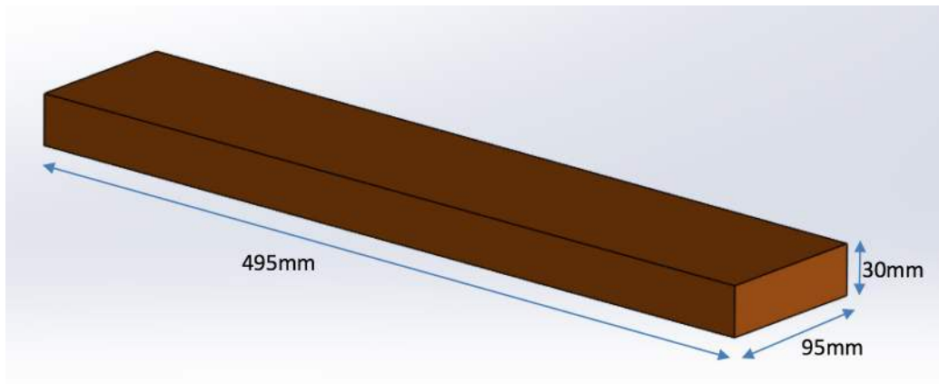
Figure 11. Dimensions for inner box packaging for LUXEON CX Plus CoB.
