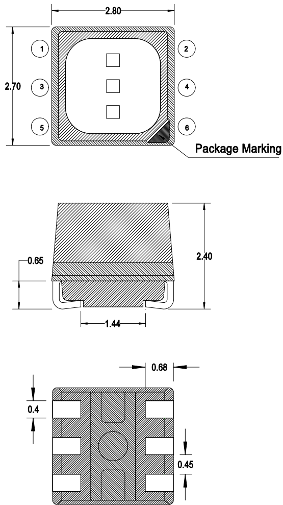
Figure 1: Package Drawing
