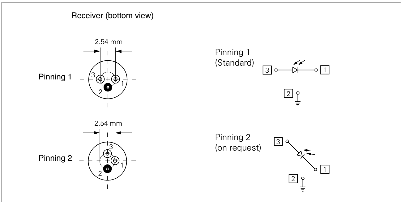
Figure 2 Receiver
