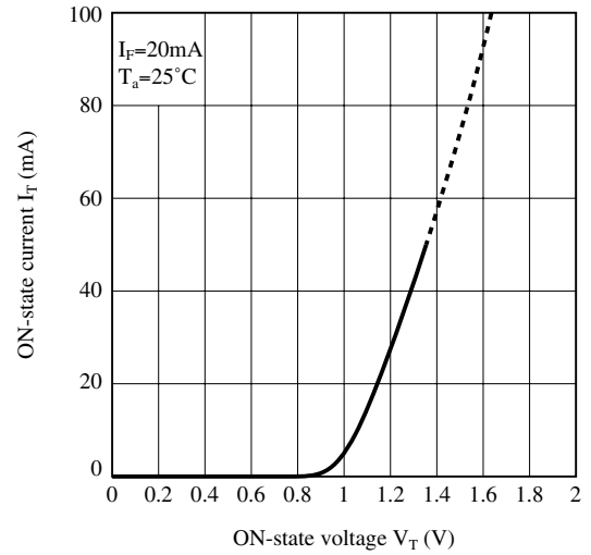
Fig.10 ON-state Current vs. ON-state Voltage
