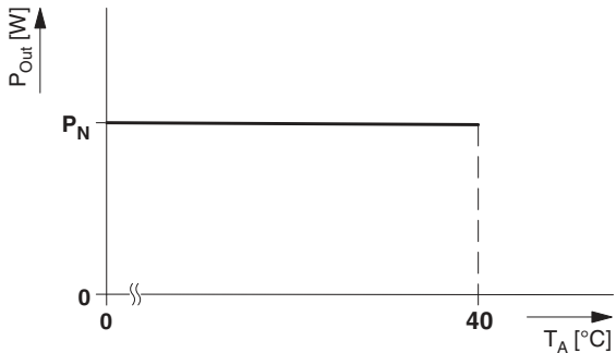
Figure 25 Temperature-dependent derating
