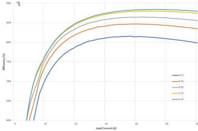
Efficiency, V_{IN} = 12V
