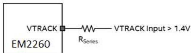
Figure 13: VTRACK Sense Circuitry (Input > 1.4V)
