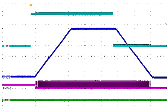
CTRL: 1 V/div, PWM: 5 V/div, V OUT : 200 mV/div, I OUT : 20 A/div
