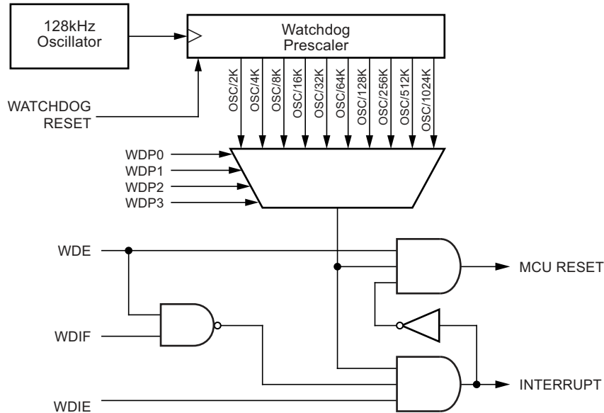
Figure 7-7. Watchdog Timer
