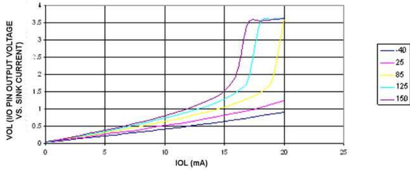
Figure 27-18. I/O Pin Low Output Voltage versus Source Current ( V_{CC} = 3V )
