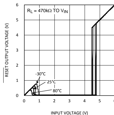
Figure 4. \overline{\text{Reset}} Output Voltage vs Input Voltage LM8365BALMF45
