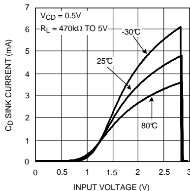
Figure 5. \overline{\text{Reset}} Output Sink Current vs Input Voltage LM8365BALMF27
