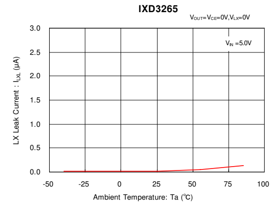
(12) Lx SW "H" Leakage Current vs. Ambient Temperature
