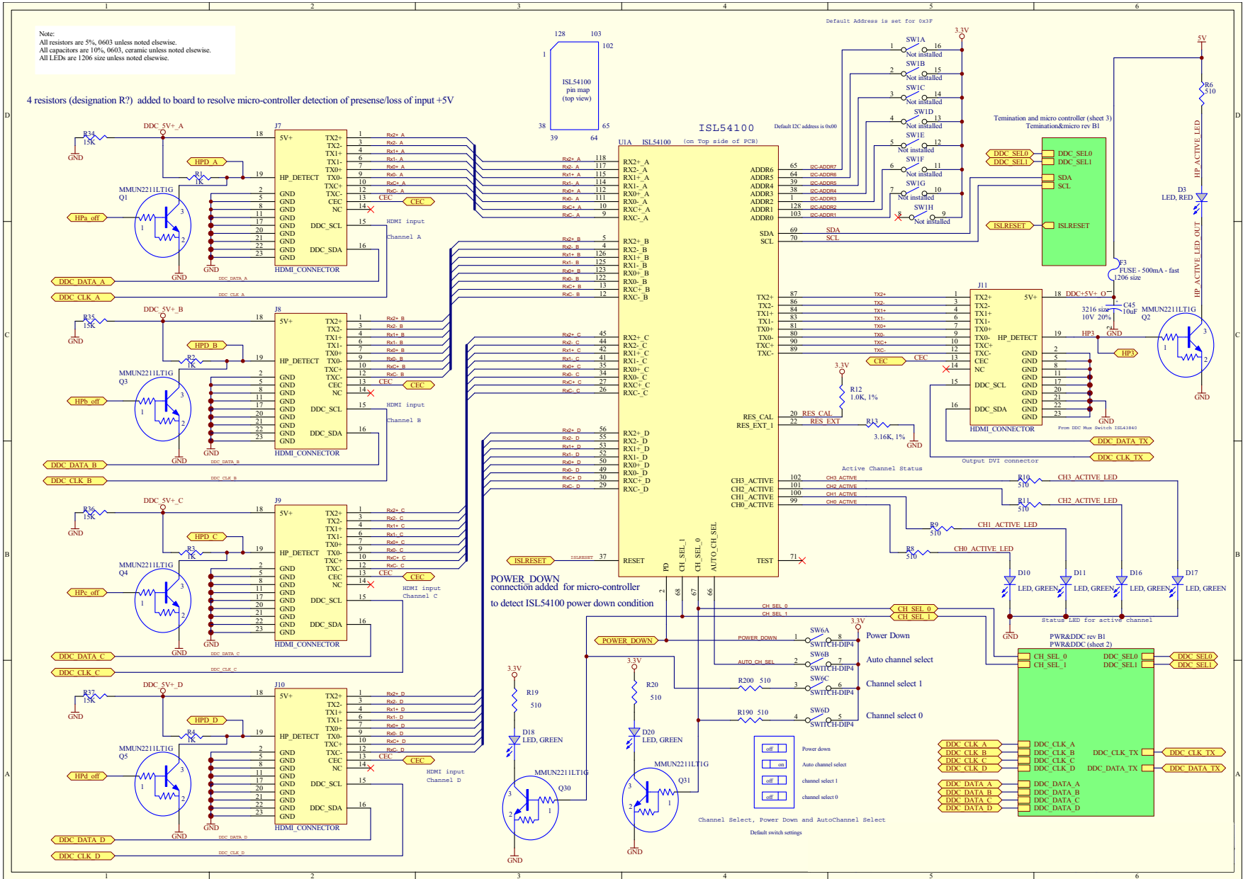
FIGURE 23. ISL54100AHDMI-EVALZ INPUT/OUTPUT
